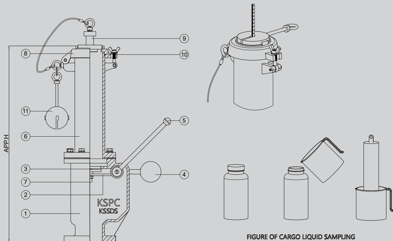
FIGURE OF CARGO LIQUID SAMPLING
